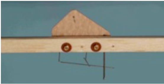
Harlan's tow hook, forward direction is to the left. The "T"-shaped fitting is the pendulum that moves forward
