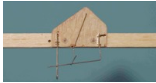
Harlan's hook from the right side of the airplane. The string from the rudder horn is attached to the small loop in the pendulum. Constructed from 0.014" music wire.
